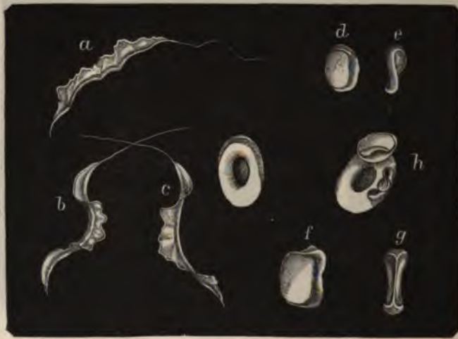
FIG. 132.—ORGANISMS IN THE BLOOD OF THE CARP.
